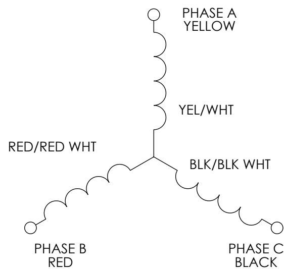
STAR WINDING TYPE
